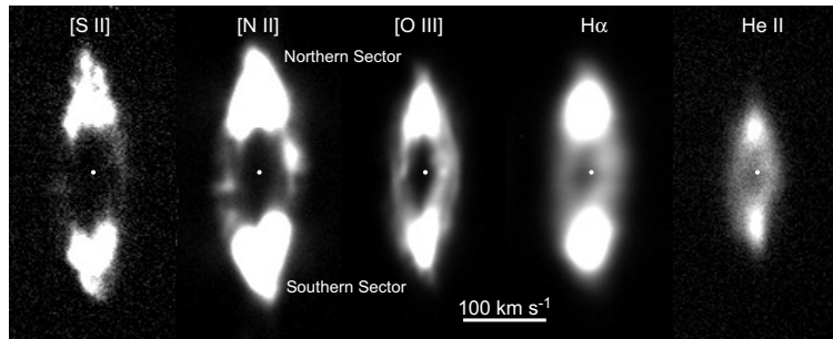
Fig. 13.— Averaged spectra over the entire nebula are shown in the same style as Figure 12, with the level of illumination set to show the features in the central region and all of the major emission-lines depicted.
