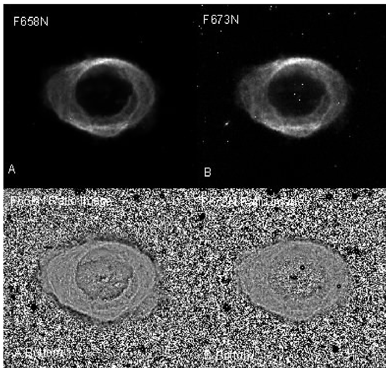
Fig. 7.— Like Figure 6 except for the F658N and F673N images.
