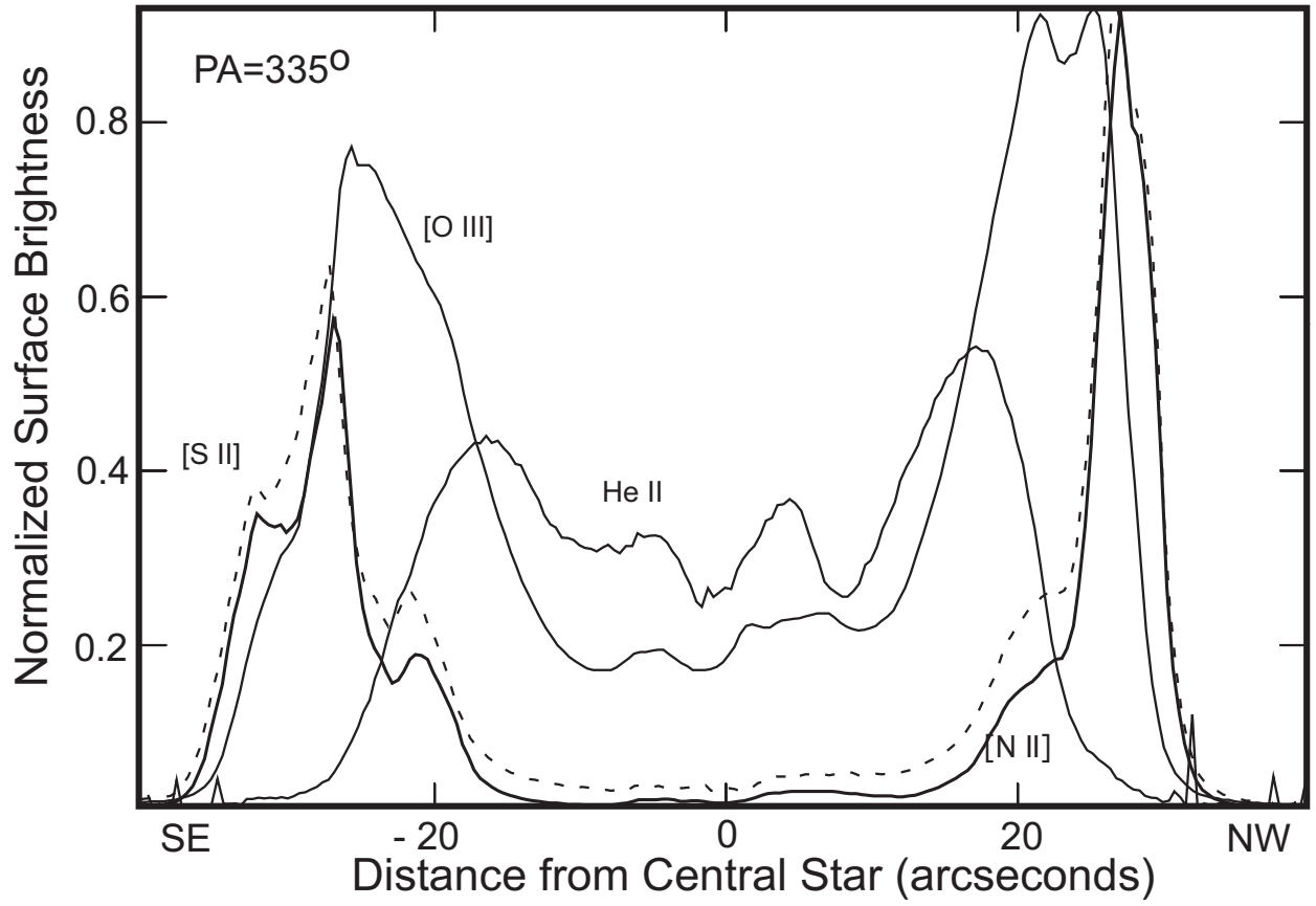
Fig. 5.— This figure was prepared in the same manner as Figure 4 except it is for the semi-minor axis profiles.
