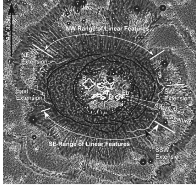
Fig. 8.— Like the individual panels of Figure 6 and Figure 7 except starting with the H_2 panel of Figure 3. The dark lines indicate the positions of arcs that lay along portions of the main ionization front seen in projection and the irregular light white lines the four regions of arcuate [N II] emission that lie outside the boundaries of the Main Ring. Open Circles show the position of [N II] bright knots that lie outside the boundaries of the Main Ring. The range of positions over which linear features (Rays) are seen in the [O III] and H_2 images are indicated. The single Ray occurring outside these boundaries is indicated by a line and occurs just above the label for the “SW Extension”. The position of the SW Blurred Feature is also shown. That feature and the Extension features are best seen in panel D of Figure 3 and bottom panels of Figure 7. The irregular heavy white solid lines (A–Eb) outline the strong Inner Region low-ionization emission features.
