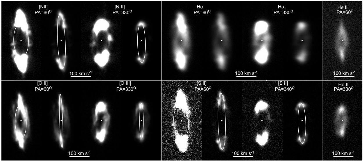
Fig. 10.— Spectra averaged over 30^\circ intervals centered on the approximate semi-major ( PA = 60^\circ ) and semi-minor axes of the Main Ring are shown for the strongest emission-lines studied, drawing on the spectra from San Pedro Mártir Observatory presented in OSH. Except for He II, the spectra are presented at two levels, left to show the faintest features and the right the brightest features. Each spectrum shows 202 \text{ km s}^{-1} along the X axis and 125'' along the Y axis.
