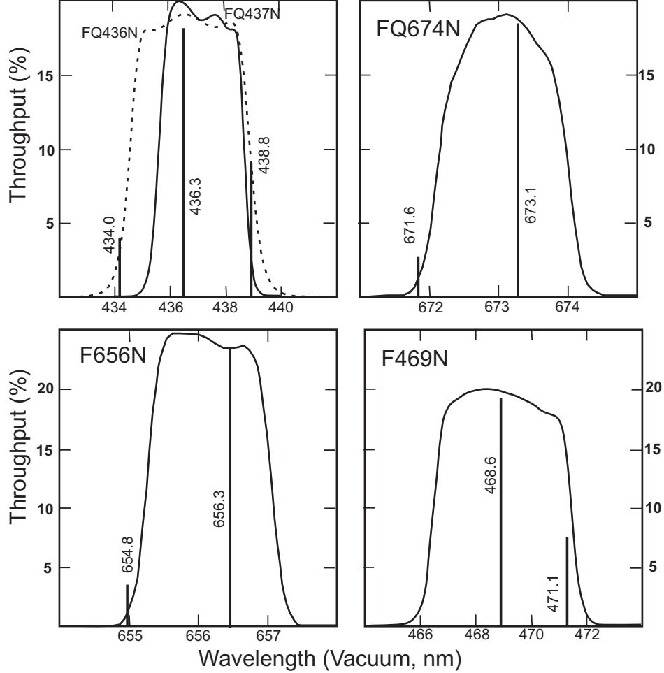
Fig. 1.— These figures each plot the Throughput versus wavelength of the fived filters in our program that are affected by contaminating emission-lines. In each case we indicate the targeted emission-line and the contaminating line(s), without an indication of their true relative values. Vacuum wavelengths were used for plotting the emission-lines, but their designations are given in the more commonly used air-wavelengths. The Throughput values are from the WFC3 Instrument Handbook Appendix A and were determined from pre-launch tests. The short wavelength profile of the filter curves will have been altered due to the convergent beam of the WFC3. The upper-left panel shows Throughput curves for the overlapping FQ436N (dashed line) and FQ437N(solid line) filters.
