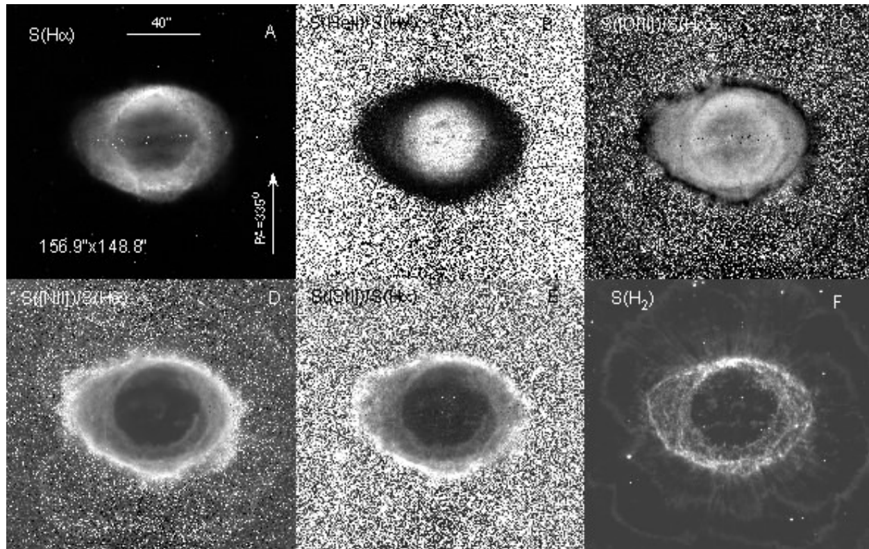
Fig. 3.— This array of images is of a 156.9'' \times 148.8'' subsample from the full field of view narrow band emission-line filters and have been corrected for contaminating lines and continuum. The “stitching” across the middle is from where the gap between the two CCDs of the detector where filled-in by dithering the pointing. Panel A presents the H\alpha image while the other panels depict ratios in various lines, except for panel F, which is a direct image in H_2 . The H_2 image was made with the Large Binocular Telescope and was provided by David Thompson.
