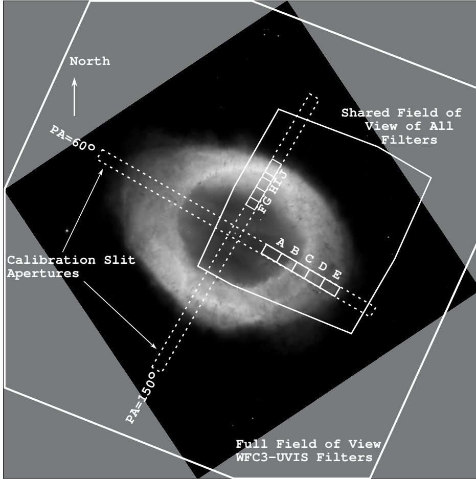
Fig. 2.— This 170'' \times 170'' image of the Ring Nebula has the vertical axis pointed towards north and is taken from the Hubble Heritage 1999-01news release of the STScI and is a composite of HST WFPC2 images in the F469N (He II), F502N ([O III]), and F658N ([N II]) filters. The outer solid lines show the limits of the WFC3-UVIS full-field filter images (F469N, F487N, F502N, F547M, F656N, F658N, and F673N). The inner solid lines show the common fields of view of the quadrant filter images (FQ436N, FQ437N, FQ575N, FQ672N, and FQ673N). The dashed-line rectangles are the slit locations for the ground-based San Pedro Martir spectra and the small solid line rectangles show the regions used in calibration of the WFC3 images.
