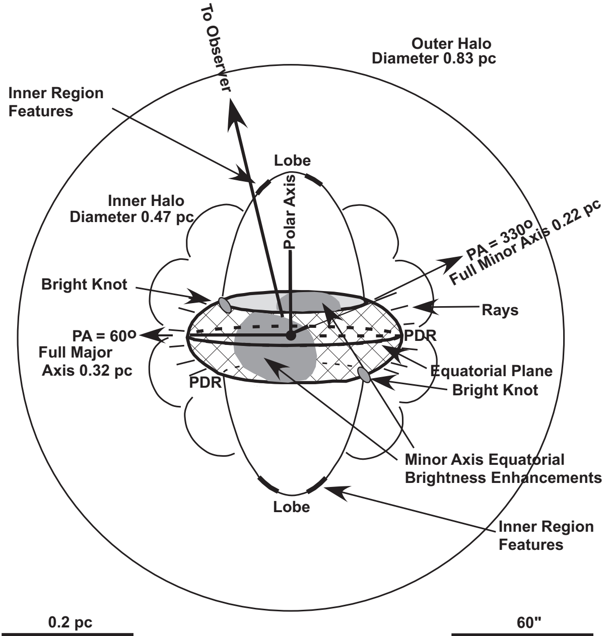
Fig. 11.— A simplified depiction of our 3-D model for the Main Ring of the Ring Nebula is shown here.
