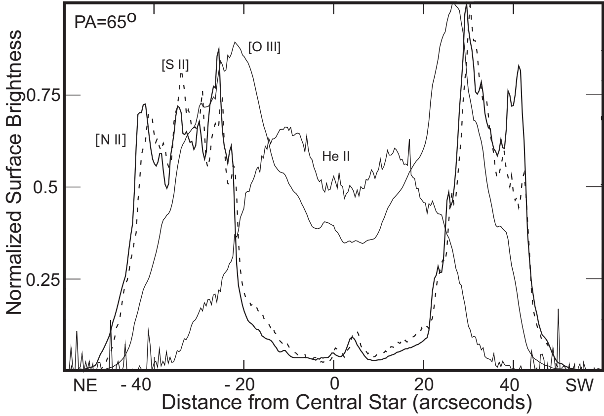
Fig. 4.— These profiles along the semi-major axis sample of the full field of view filters depict the strongest emission-line of each ion. Again the samples were 4'' wide and were averaged in 0.4'' bins. The data are normalized to peak values near unity, except for He II, which is normalized to a lower value for clarity. The dashed line indicates the sum of the [S II] 671.6 nm + 673.1 nm emission-lines.
