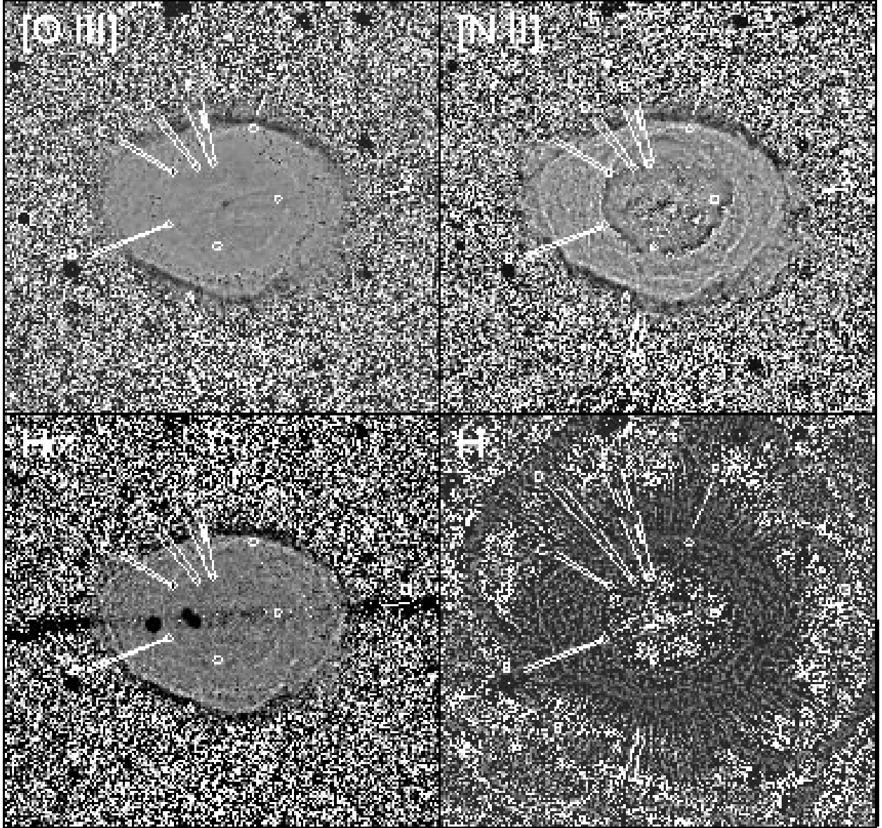
Fig. 9.— Like the bottom panel of Figure 6, Figure 7 A, and Figure 8, with the addition of a similarly processed H\alpha image. The features are designated A-G in counterclockwise notation with the PA values being A( 142.6^\circ ), B( 65.8^\circ ), C( 34.2^\circ ), D ( 13.2^\circ ), E( 352.5^\circ ), F( 315.1^\circ ) and G( 248.8^\circ ). The solid lines outline the boundaries of the feature and the open circles indicate the associated dark knots. Narrow straight dashed lines indicate enclosed narrow dark features seen in the F502N images and the cross-hatched region within object E indicates an extended region dark in the F502N images. The heavy dashed line indicates the position of the [O III] portion of feature A. In both the [N II] and H_2 images the wavy light line in feature A indicates the associated bright H_2 emission and in the [N II] image the light solid line indicates the [N II] emission. Full resolution images are given in the electronic version of this paper.
