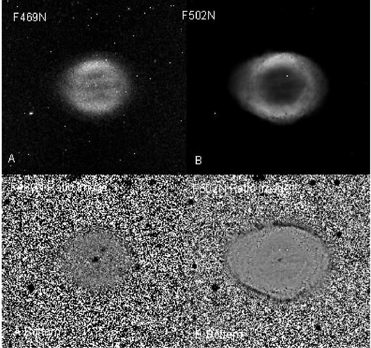
Fig. 6.— The same FOV as Figure 3 is shown in each panel. Panels A and B are the images in the F469N and F502N filters. Panels A Bottom and B Bottom are the upper images divided by a gaussian blurred version of itself with a FWHM of 2.00'' . The ratio images show best the fine scale structure.
